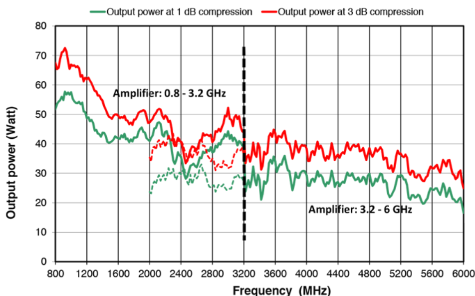
SX40/30 POWER AMPLIFIER 40W-30W / 800 MHz - 6000 MHz
