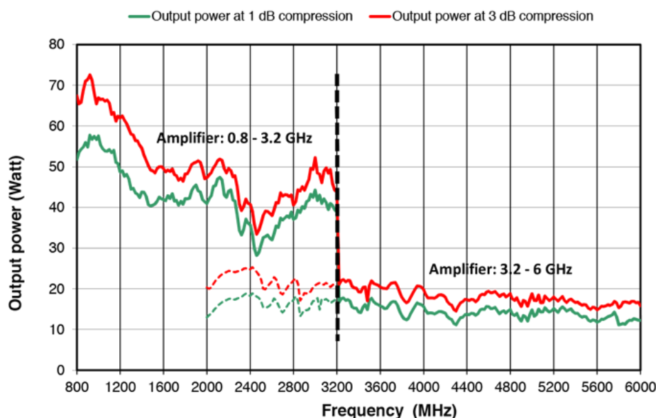
SX40/15 POWER AMPLIFIER 40/15W / 800 MHz - 6000 MHz
