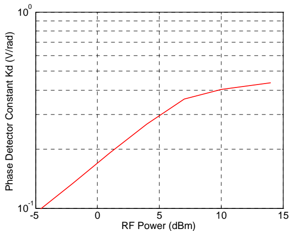
Figure 9: K D (V/rad) vs. RF Power (K D = Phase Detector Constant)
